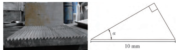
图 1 钢制模具图及锯齿示意图 Fig.1 Schematic diagram showing the steel mould and sawtooth
